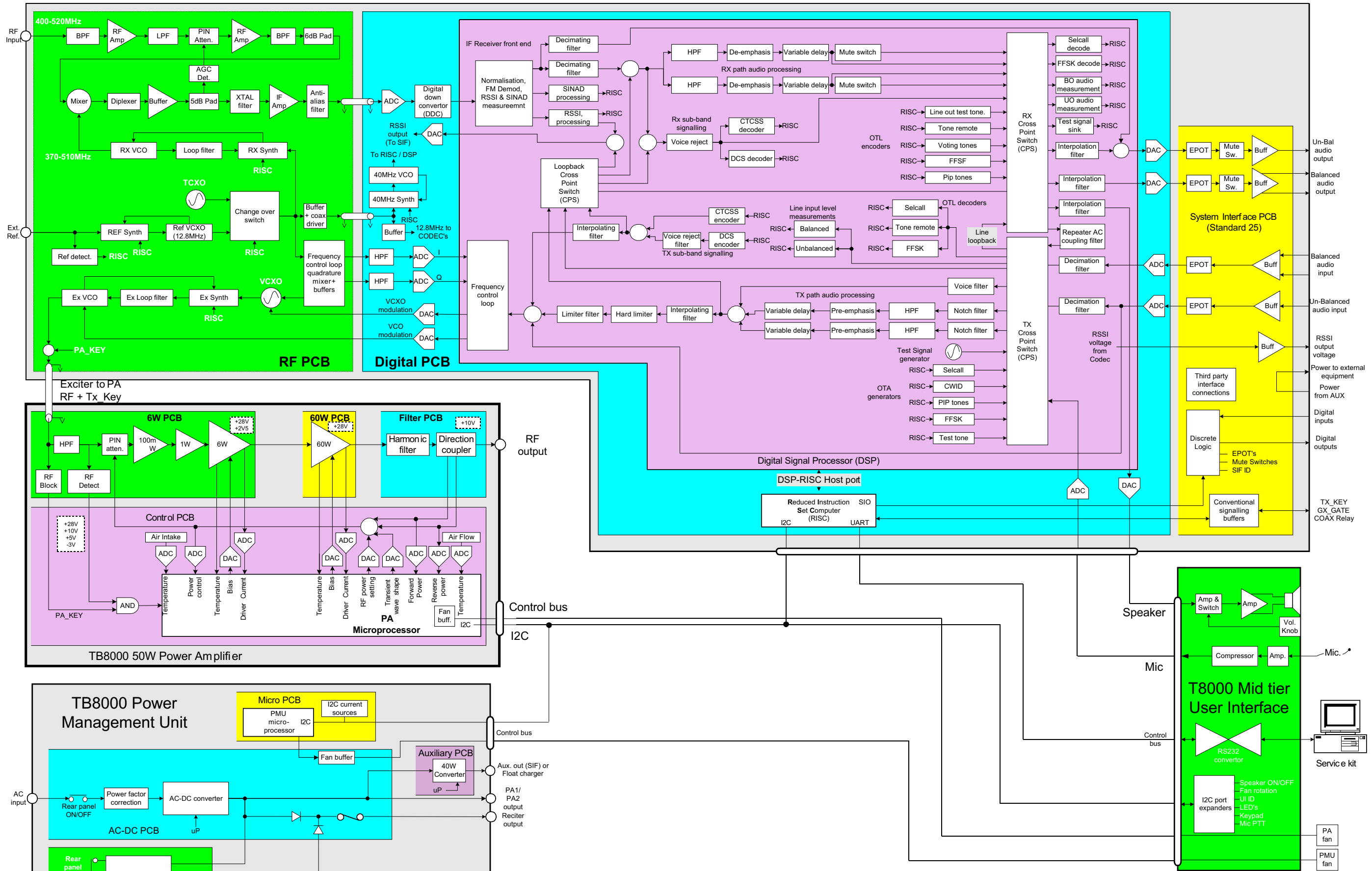
TB8000 Signal Path Diagram
